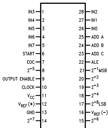
Figure 2. Dual-In-Line Package
