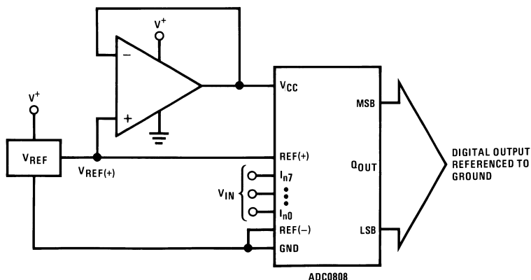
Figure 14. Ground Referenced Conversion System with Reference Generating V_{CC} Supply
