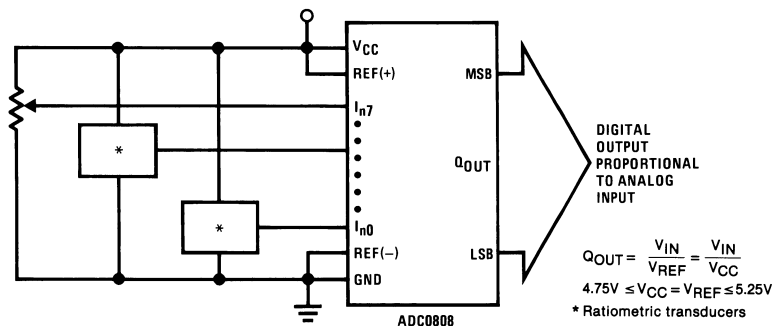
Figure 12. Ratiometric Conversion System
