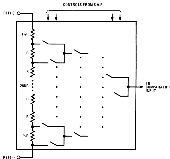
Figure 4. Resistor Ladder and Switch Tree
