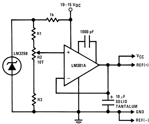
Figure 15. Typical Reference and Supply Circuit
