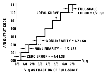
Figure 5. 3-Bit A/D Transfer Curve
