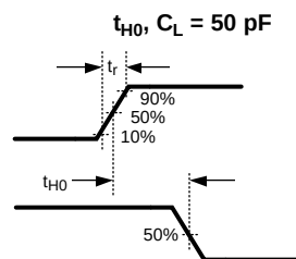
Figure 11. TRI-STATE Test Circuits and Timing Diagrams
