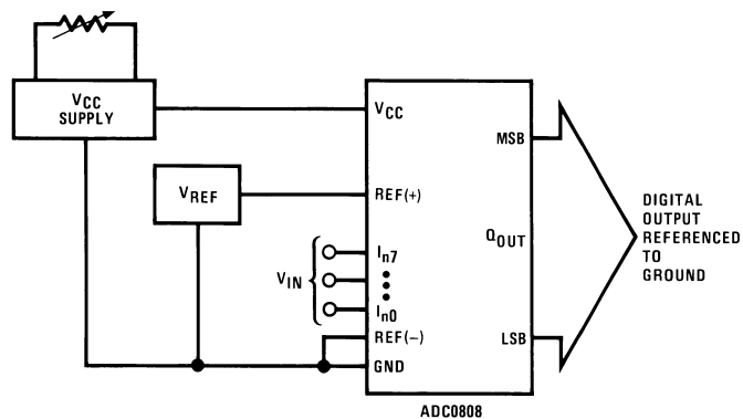
Figure 13. Ground Referenced Conversion System Using Trimmed Supply
