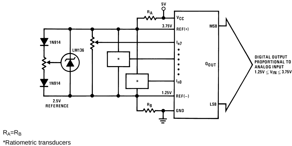
Figure 16. Symmetrically Centered Reference
