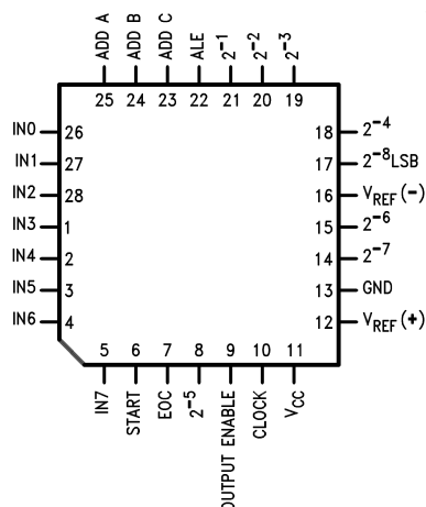
Figure 3. Molded Chip Carrier Package
